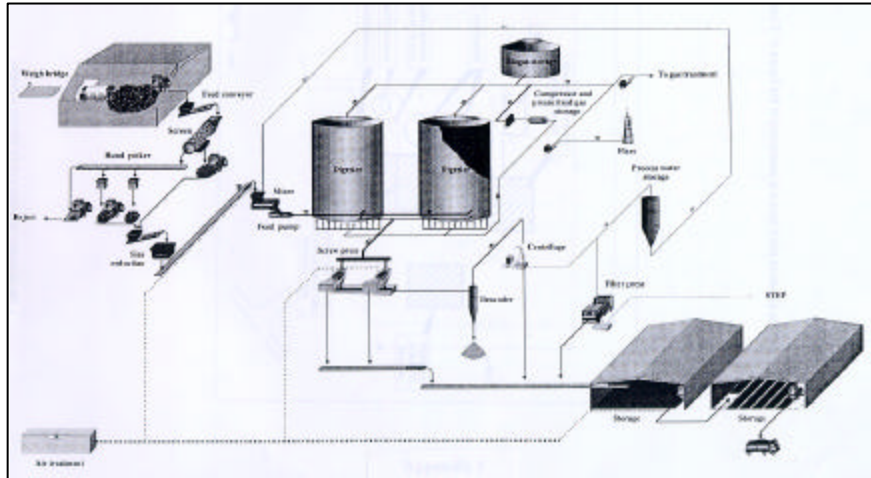
Principle sketch of the VFG digestion plant
